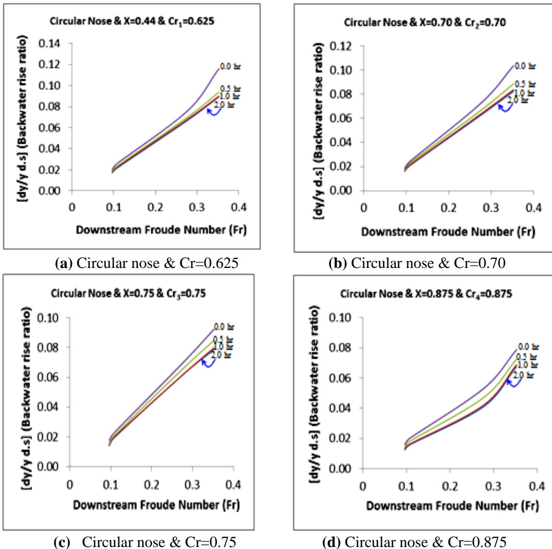
Figs. 10 Effect of time on backwater rise ratio for circular nose at different values of Cr.
