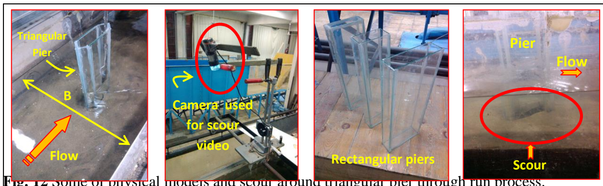
Fig. 12 Some of physical models and scour around triangular pier through run process.
