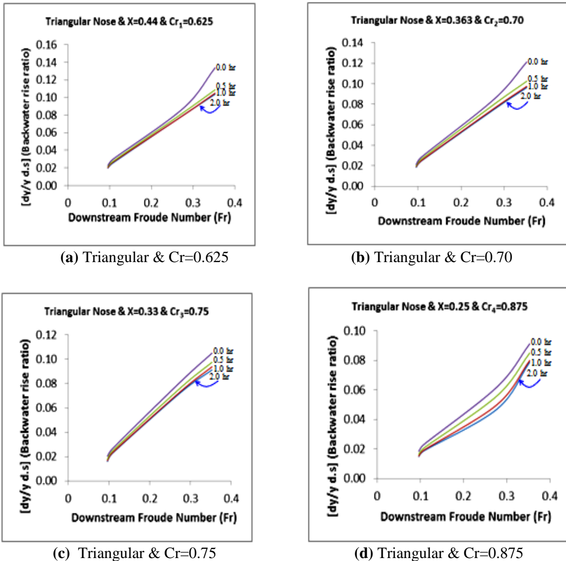
Fig. 11 Effect of time on backwater rise ratio for triangular nose at different values of Cr .
