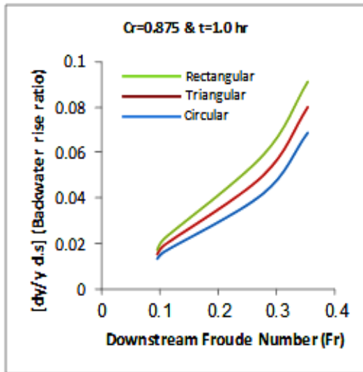
Fig. 7: Backwater rise ratio at t=1.0 hr.
