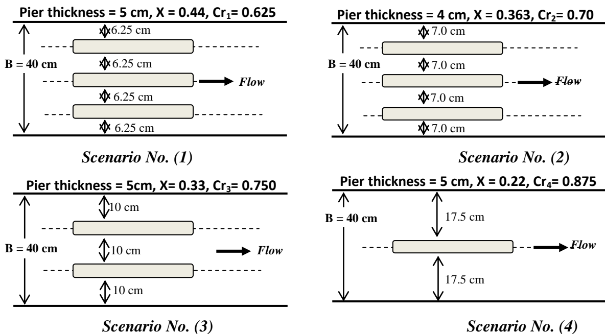
Fig. 4 Sketch for the used models scenarios.
