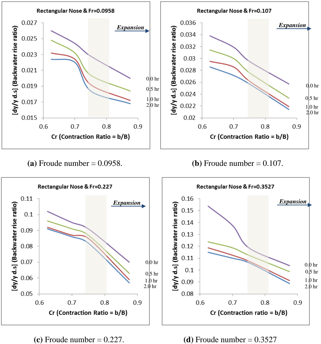
Fig. 9 Relationship between [dy/y_{d.s}] and Cr for different Froude numbers.
