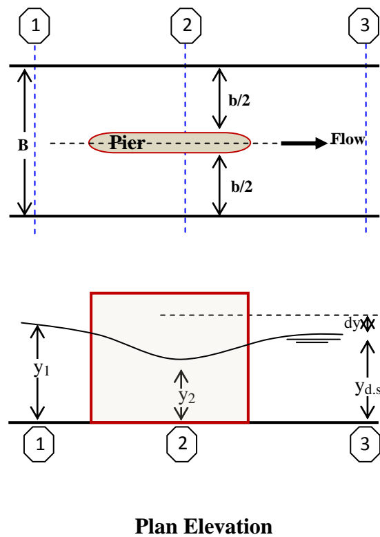
Fig. 1 Backwater rise due to bridge piers ( dy ).
