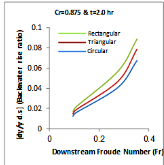
Fig. 8 Backwater rise ratio at t=2.0 hr.
